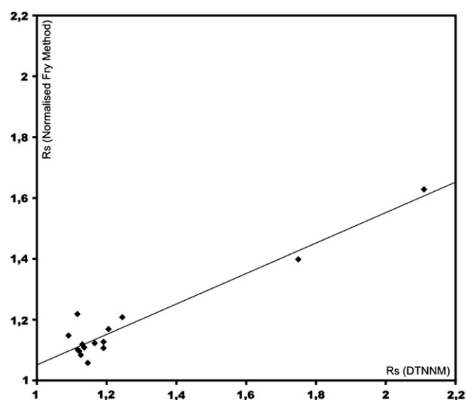
Fig. 4. Plot of the strain measured with DTNNM versus Normalised Fry Method in the samples with very low or no matrix content, where DTNNM works correctly. Normalised Fry Method shows a little R_s underestimation. Linear regression is used, showing an R^2 of 0.92.
